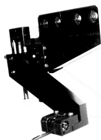
Micro-Force carbon Si Tun cantilever for contact fiber profilometry
