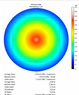
Wafer stress bow & warp calculation
