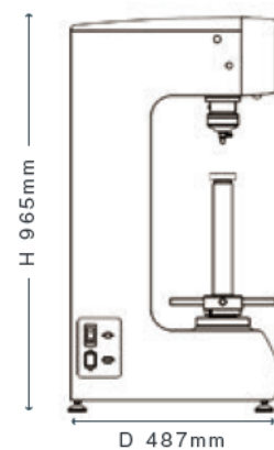
□ Left view
