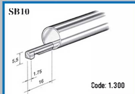
SB10 - Standard probe for plane surfaces or diameters internal/external larger than of 10 mm.
