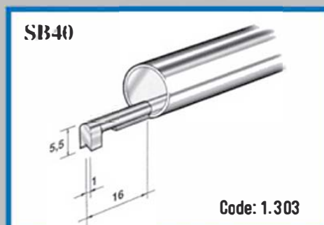
SB40 - "V" skid, for wires, and cylinders with external diameter more than 1 mm.
