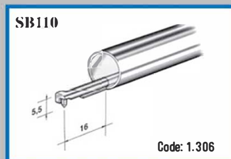
SB110 - For concave and convex surfaces with minimum radius of 5 mm.
