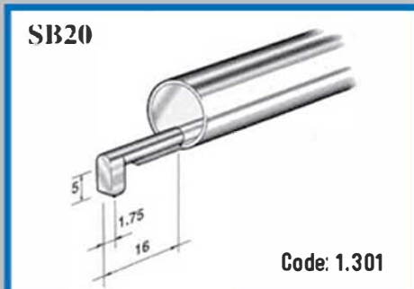
SB20 - For plane surfaces, grooves and shoulders with depth up to 5 mm.
