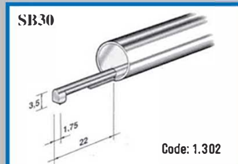
SB30 - For planes and holes with diameters more than 4mm and deep up to 20mm.
